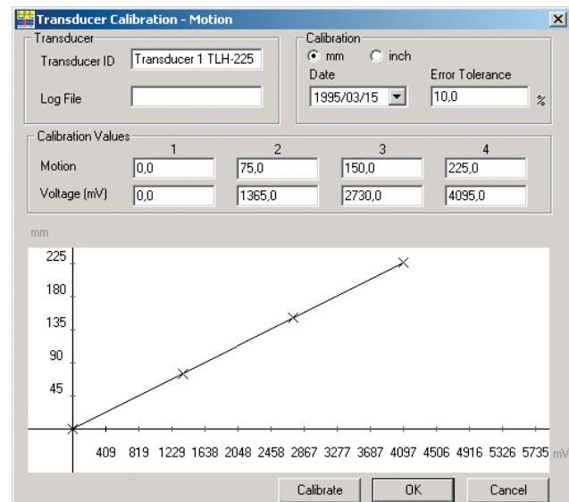
Figure 2. Linear and angular travel, voltage, current, pressure and vibration transducers can be defined and calibrated with CABA Win
